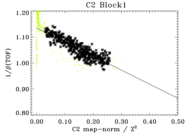
Fig. 1. 1/\beta_{TOF} versus C2 map-normalized signal divided by the square of the charge for beryllium, carbon, and oxygen events. The y-intercept gives the index-of-refraction ( n = 1/\beta ).
