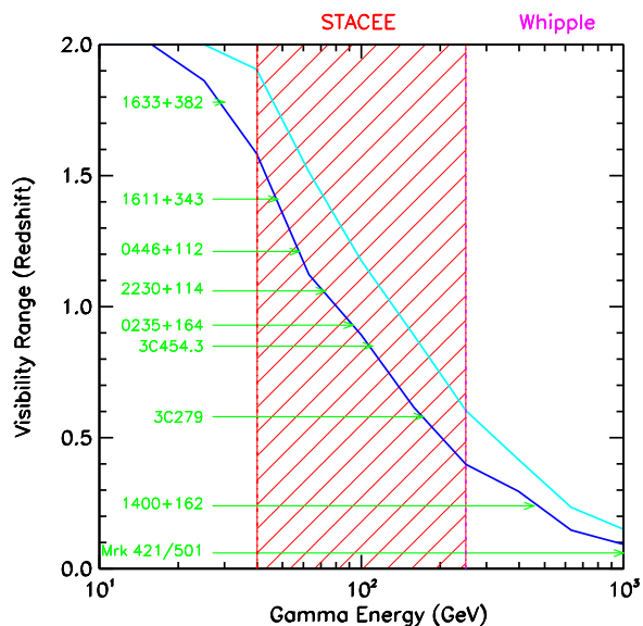
Fig. 1. Expected \gamma -ray horizon as a function of energy. The horizon results from the absorption of \gamma -rays by diffuse radiation in intergalactic space. The two lines running diagonally represent the range of plausible cosmic infrared background models (see text for details). As distance increases, lower energies are required to permit detection of the source. Current Cherenkov imaging telescopes, such as Whipple, CAT, and HEGRA, are likely to detect only the closest AGN. New low-threshold ( \sim 50 GeV) experiments, such as CELESTE and STACEE, have the potential to detect many more sources.
