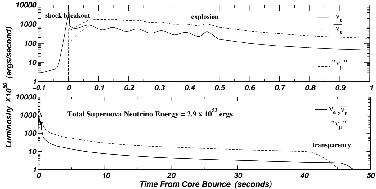
Fig. 1. Luminosity evolution from the model of Burrows et al. (Burrows et al. 1992) used in the SNO supernova Monte Carlo.
