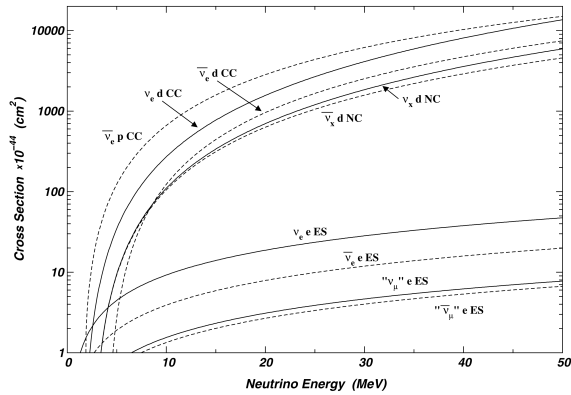
Fig. 2. Supernova neutrino cross-sections relevant to the SNO detector.
