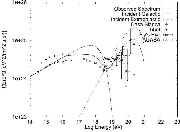
Fig. 1. The cosmic ray spectrum f(E) multiplied by E^3 for E > 10^{14} eV. Long and short dashed lines are respectively the incident galactic and extragalactic components. Solid line is the combined spectrum expected to be measured for y = 1/2 , \alpha = 2 . +’s are the Tibet data, diamonds the Casa Blanca data, squares the Fly’s Eye data and \times ’s the AGASA data.
