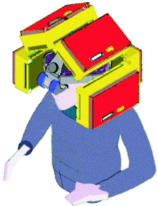
Fig. 1. A schematic view of the astronaut with the ALTEA system (frontal unit not shown).
