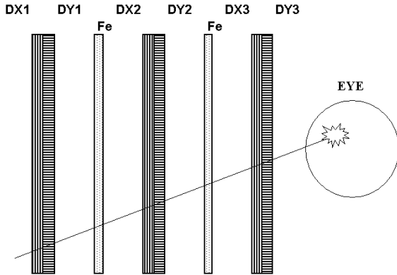
Fig. 1 The SilEye-2 detector. The three planes of double silicon layers are interleaved with two 1-mm iron absorbers.
