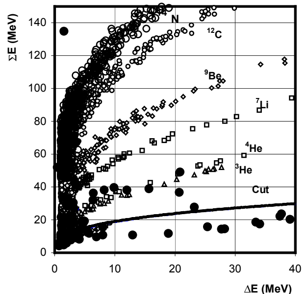
Fig. 2. \Sigma E vs. \Delta E scatter plot from a SilEye-2 detector simulation.
