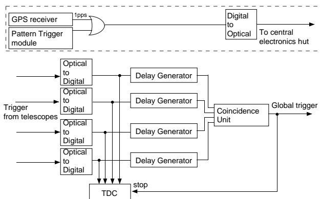
Fig. 5. Global trigger of four telescopes. The area enclosed with dash lines shows a local trigger of each telescope.
