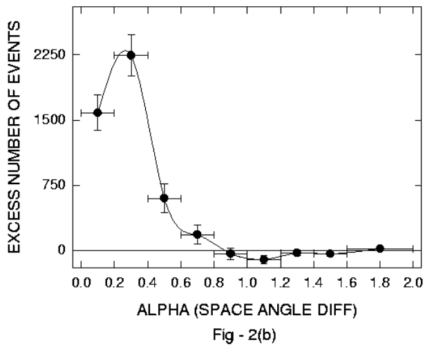
Fig. 2. (a) \alpha distributions for events in data source(upper) and background (lower) (b) The excess number of events v/s \alpha .
