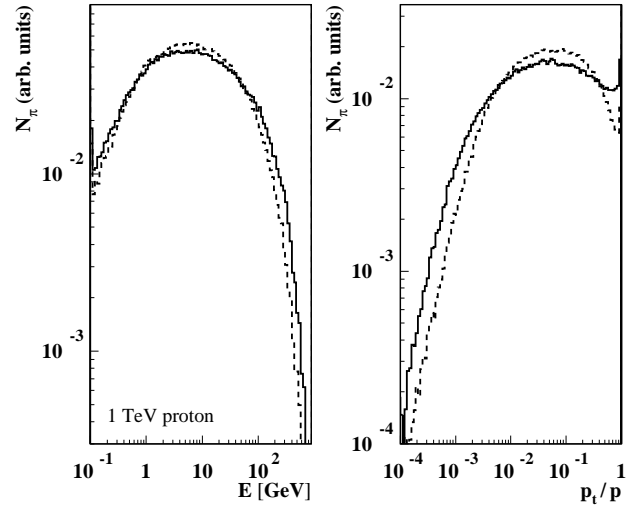
Fig. 2. Same as figure 1, but for collisions generated by 1 TeV protons.
