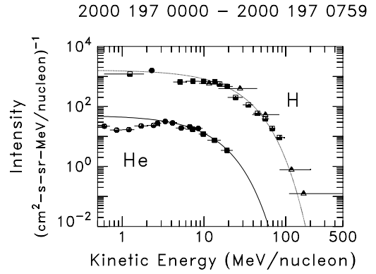
Fig. 6. (from Tylka et al. 2001): H and He in the Bastille Day event from GOES (half-filled triangles, H only), Wind/LEMT (filled circles), IMP8/GME (filled squares), IMP8/CRNC (half-filled squares, H only), and ACE/EPAM (half-filled circles, He only). Curves are exponentials, with e-folding energies scaled from that of carbon in Fig. 1, as described in the text.
