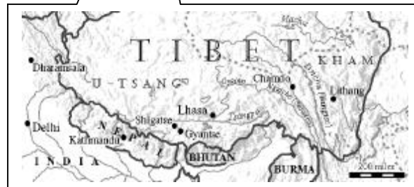
Fig. 1 - Location of the Italian-Chinese ARGO-YBJ experiment.
