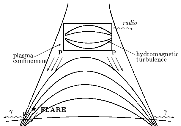
Fig. 1. Schematic picture of plasma confinement in a coronal loop, formed well after the flare. The \gamma rays are assumed to be produced both at the time of the impulsive phase and during the gradual phase when accelerated particles are dumped into the solar atmosphere. The radio emission is supposed to be produced by the confined plasma.
