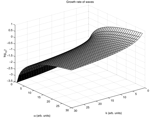
Fig. 4. Numerical calculation of the growth rate of waves, expression (3), as a function of wave number k and frequency \omega
