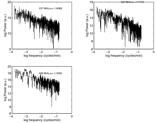
Fig. 3. Power spectra of the temporal evolution of the radio emission at 237, 327 and 408 MHz as observed at the Trieste Observatory for the delayed phase of the event of 15 June, 1991
