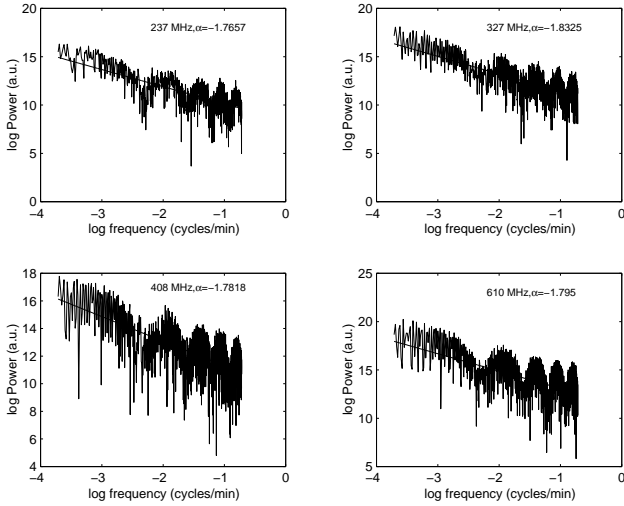
Fig. 2. Power spectra of the temporal evolution of the radio emission at 237, 327, 408 and 610 MHz as observed at the Trieste Observatory for the delayed phase of the event of 29 September, 1989
