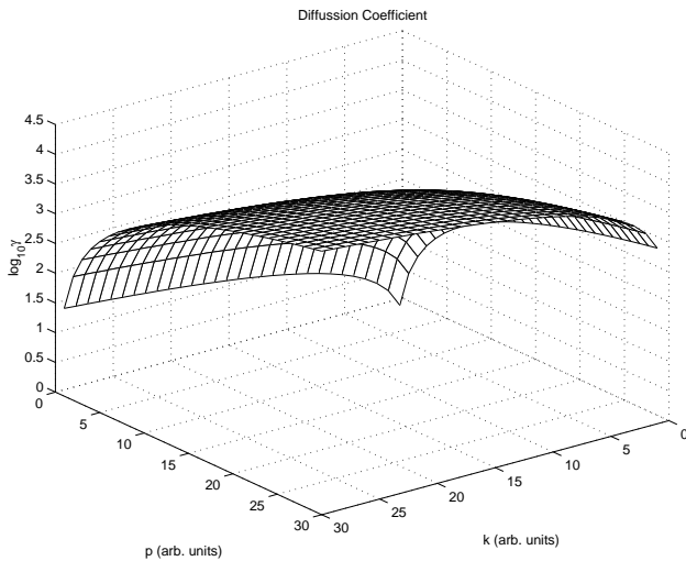
Fig. 5. Numerical calculation of the diffusion coefficient in momentum space, expression (2), for high frequencies. Both k and p are in arbitrary units.
